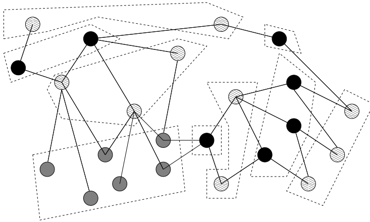
FIG. 1. An example of a graph in \mathcal{G}_n .
